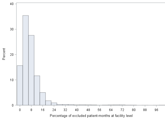
Figure 1. Histogram of patient-months excluded, at facility level, 2016
